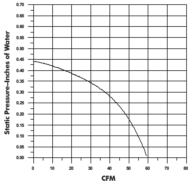
NuVent Product Performance Model NXPF50
